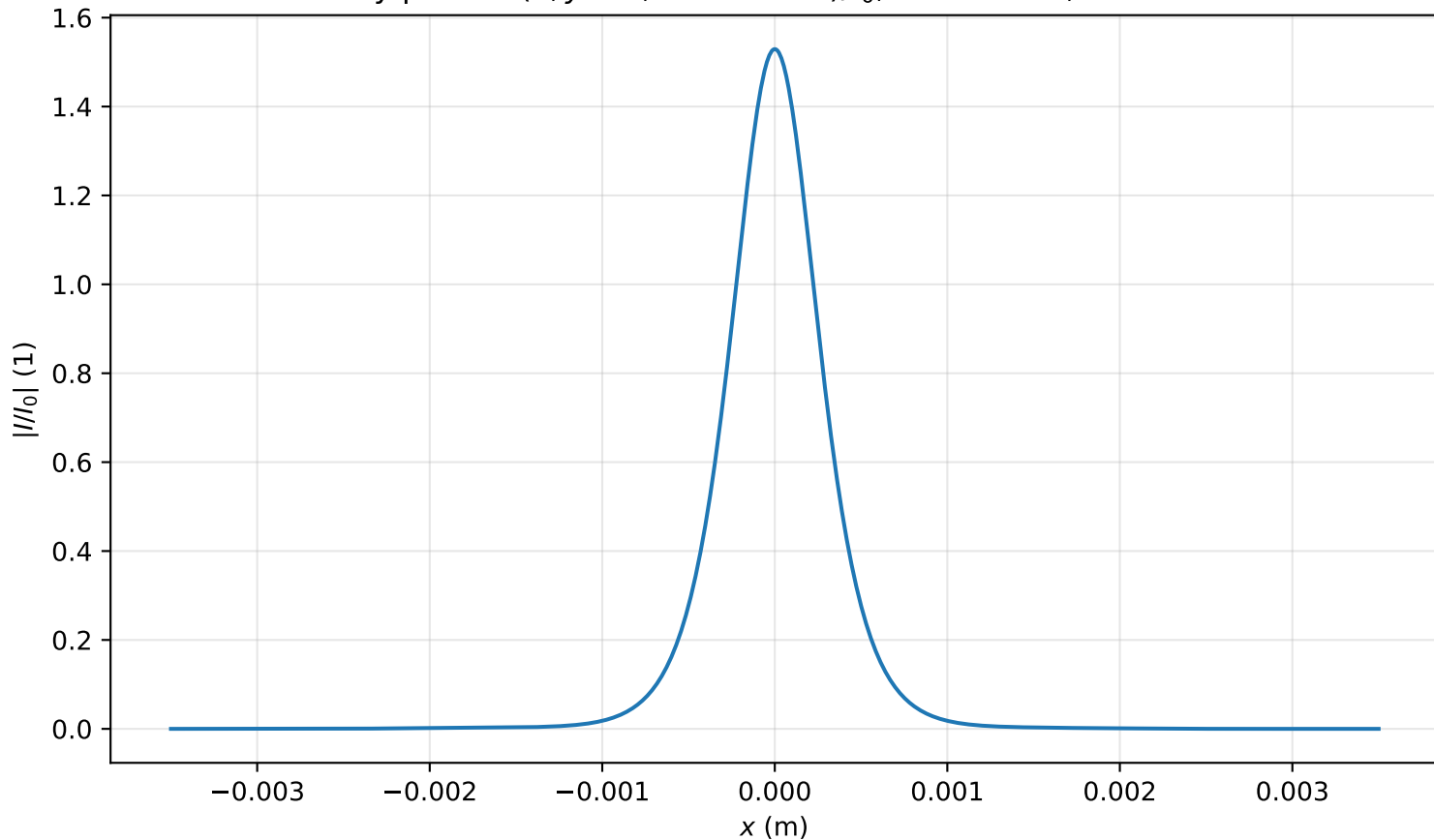
Intensity profile I(x, y = 0, z = 3.264m)/I_0 , P_{in}=0.9P_{cr} , artificial time
